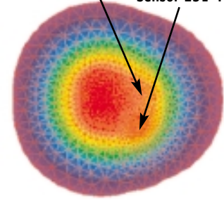
Process Tube 232°F Factory Installed Sensor 231°F
