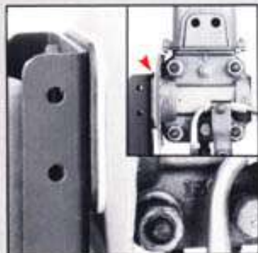
The unique spacer greatly reduces the amount of heat lost from the instrument through the mounting bracket and pipe stand.
