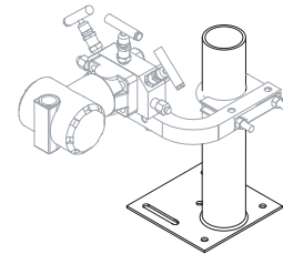
MANIFOLD MOUNTING
