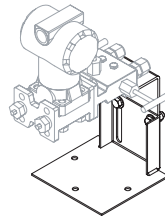
TRANSMITTER MOUNTING
