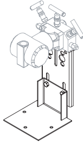
MANIFOLD MOUNTING
