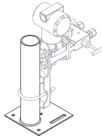
MANIFOLD MOUNTING
