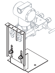
TRANSMITTER BACK MOUNTING
