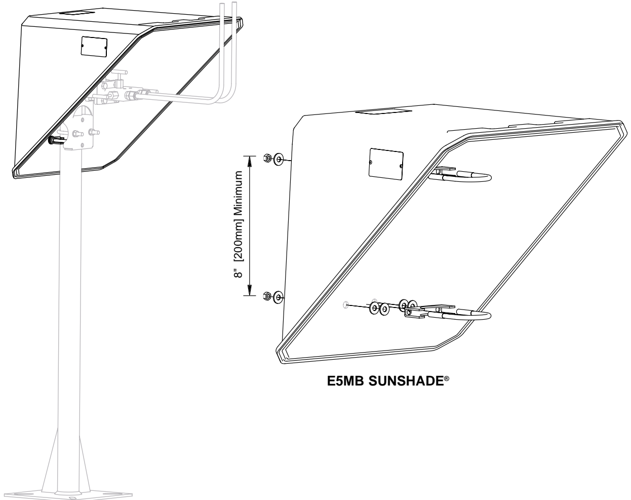
E5MB SUNSHADE® MOUNTED ON SADDLEPAK® STAND
